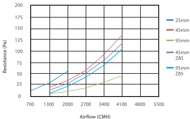
Clairo Carb Z - Airflow vs. Initial Resistance
